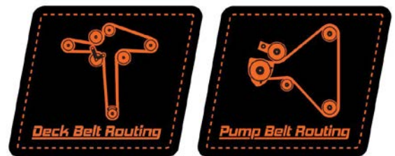
491-0082-00 Mower TTQ Deck Belt and Pump Routing Decal
